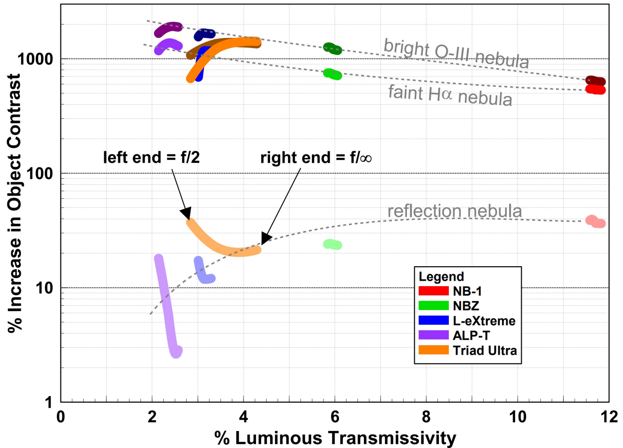
Figure 9 Predicted Filter Performance: Back Illuminated Colour CMOS, LP w/LED (NELM+2.9)
